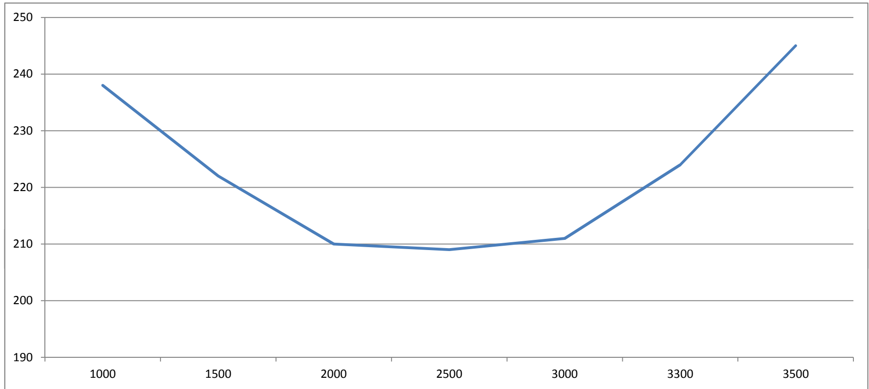
MDVGT500 BSFC g/kWhr
